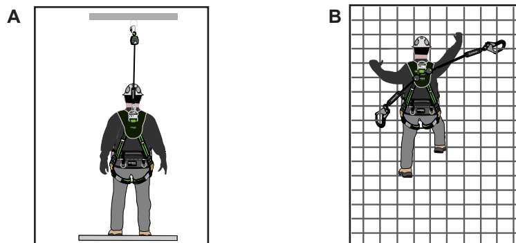
FIGURE 6 - SYSTEM CONNECTIONS
